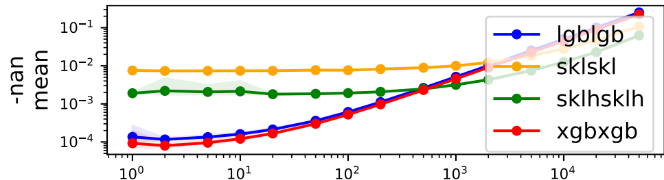
dataset=breast_cancer
