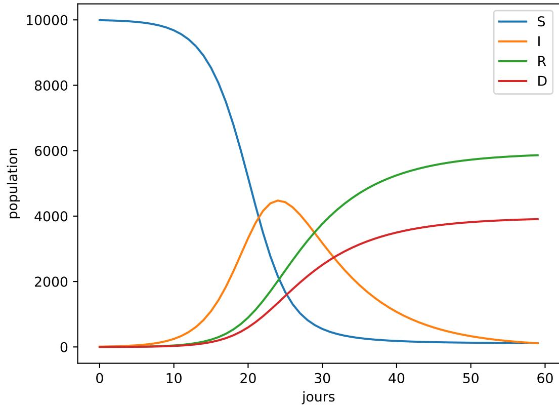
Simulation SIRDC R_0=4.200000
